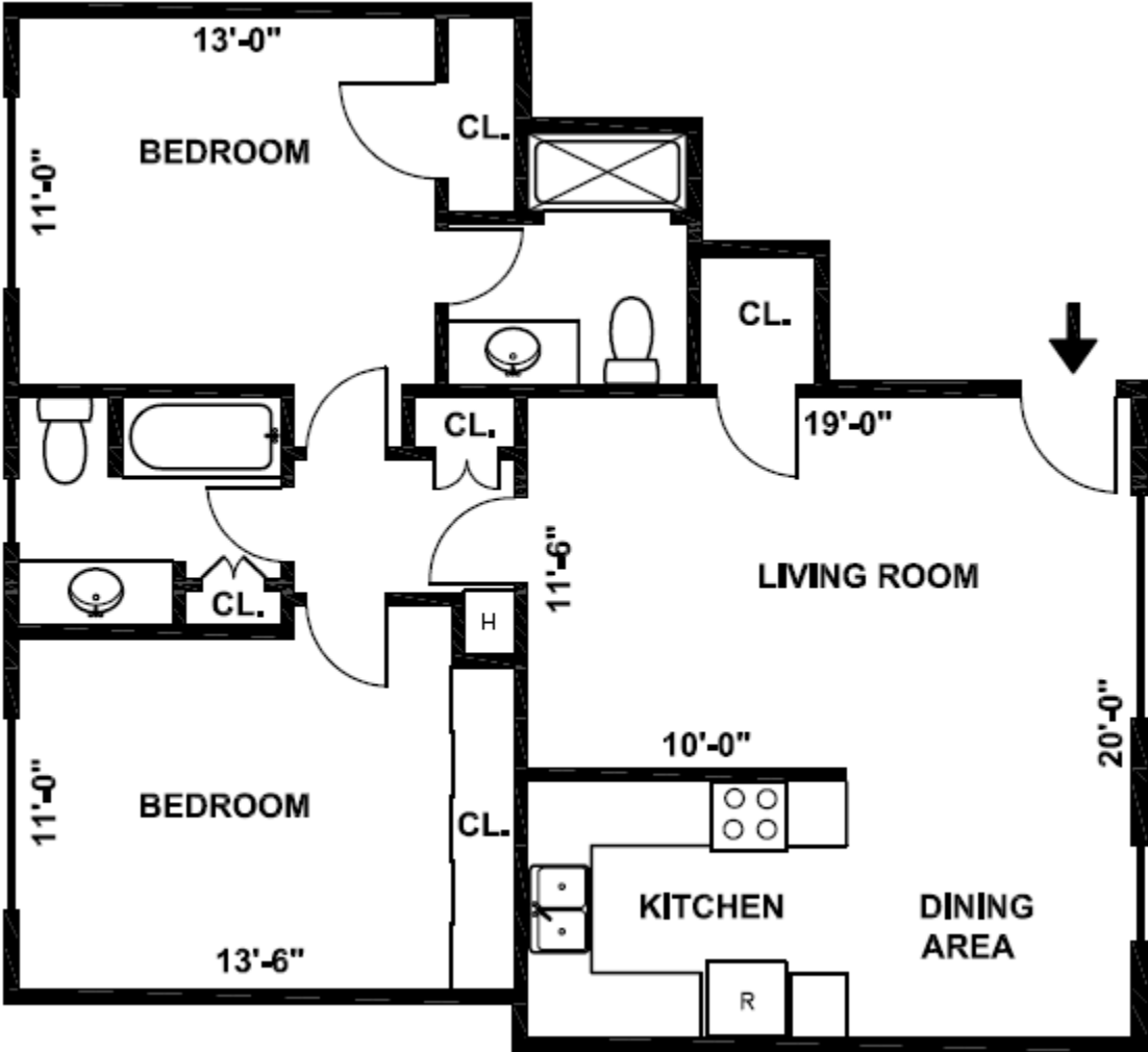
2 Bedroom – Sample Floorplan
