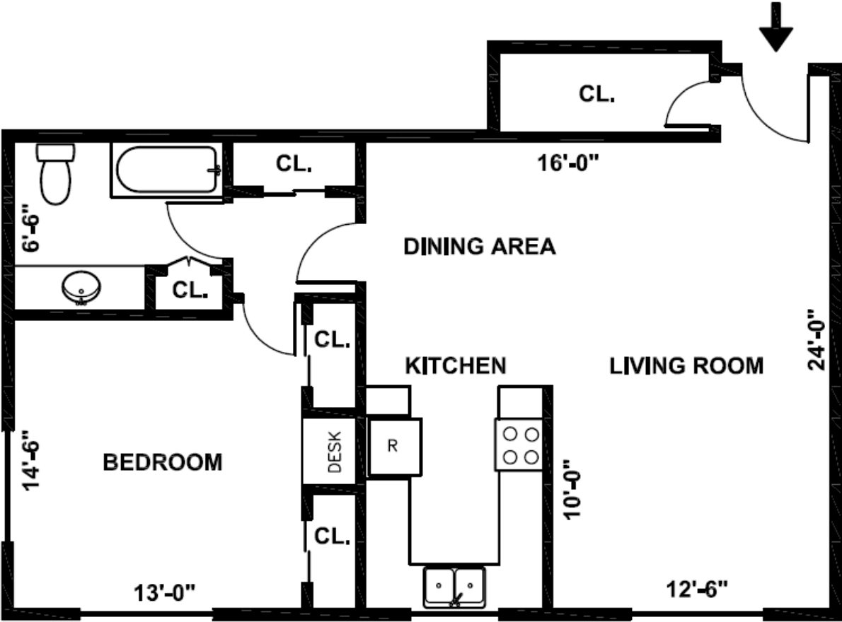
1 Bedroom – Sample Floorplan
